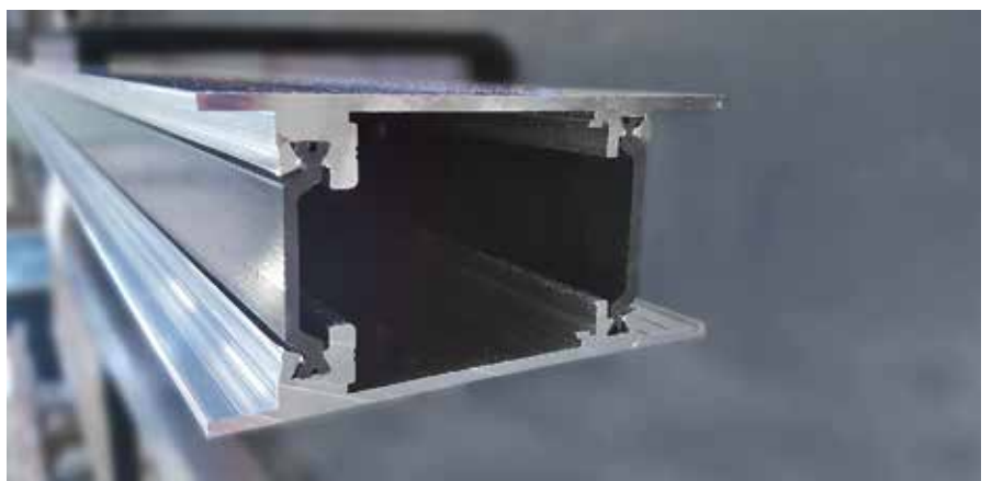
Thermally separated lightweight profile TORMAX LR 32THERM
